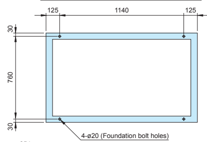
Vibration Isolation Platform Foundation Bolt Locations *Viewed from above.
