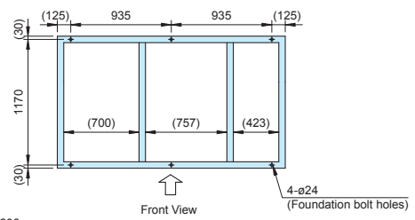
Vibration Isolation Platform Foundation Bolt Locations *Viewed from above.
